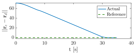
(a) 2-norm distance between \mathcal{E} and \mathbf{r}_d
